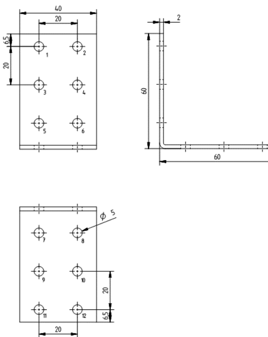
Figure A.10 Angle Bracket 8593 6060 1
