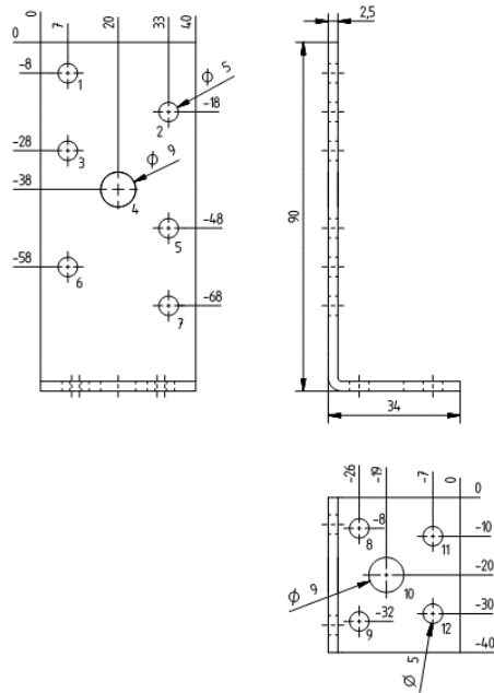
Figure A.62 hold-down 8795 0090 1FH
