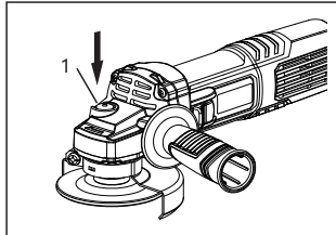
1.Spindle Lock
