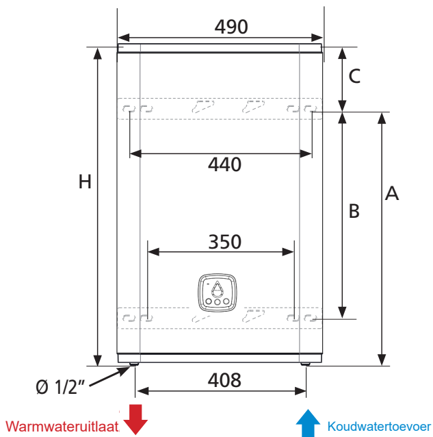
Verticale wandboiler
