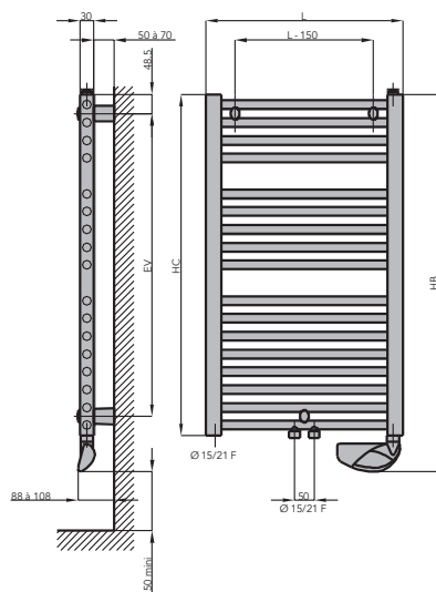
VERSION MIXTE* (...MA)
