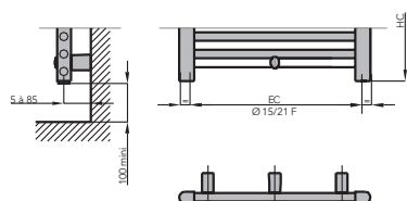
VERSION EAU CHAUDE STANDARD (...SEC)
