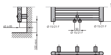
VERSION EAU CHAUDE RACCORDEMENT CENTRAL 50 MM (...SEC5)
